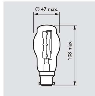
BTT46 B22d / 25 26
