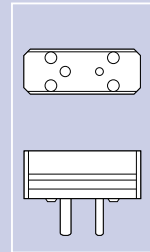
GY16 IEC: 7004-74
