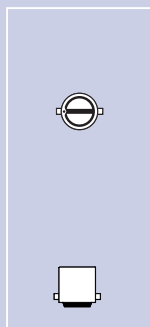
BA15d DIN:49720 IEC: 7004-11A ANSI: Candelabra bayaonet base double contact C 81-30-1976 sheet 1-3-1
