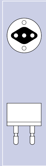
G22 IEC: 7004-70-1 ANSI: Medium bipost
